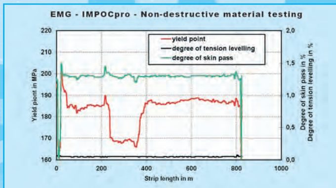
Optimizing of the operating process with IMPOCpro
