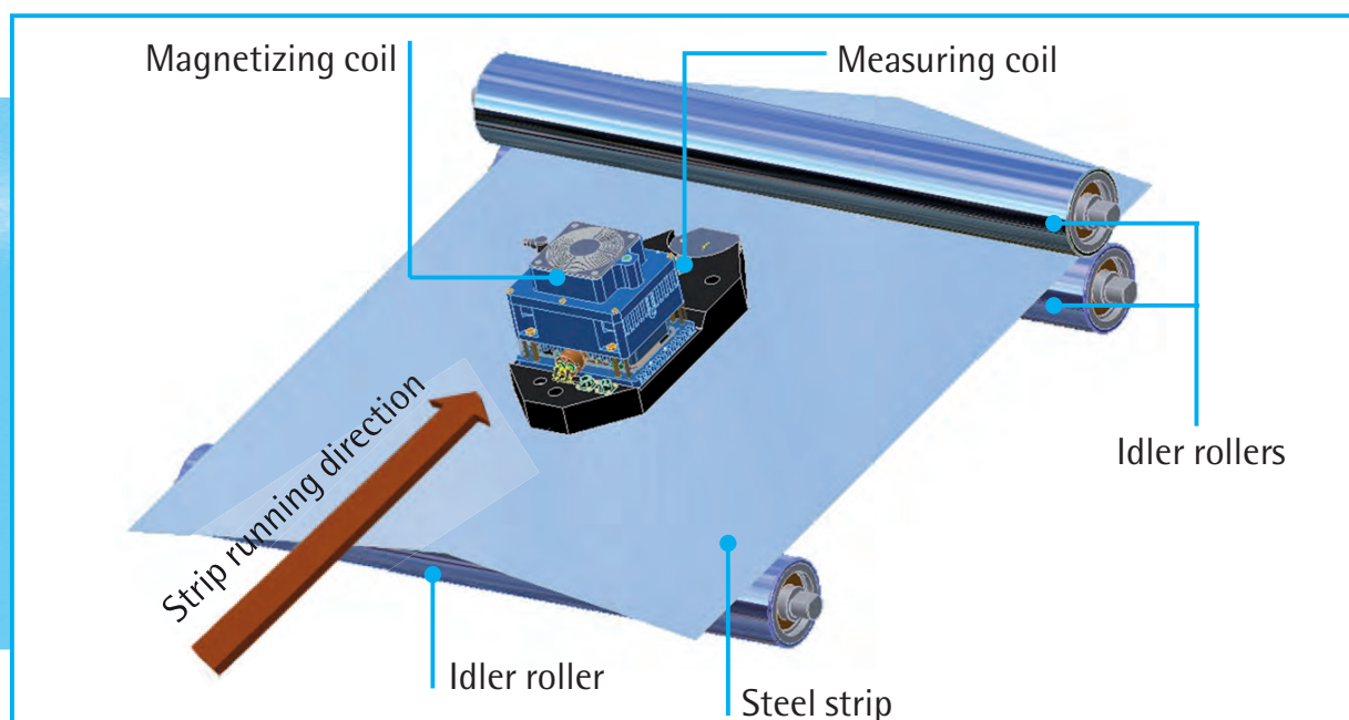
Scheme of the operating principle of IMPOCpro
